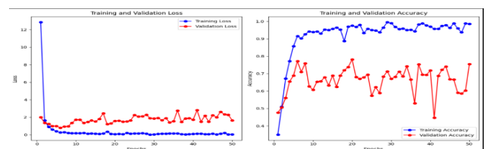
Figure 6. ResNet-50.
